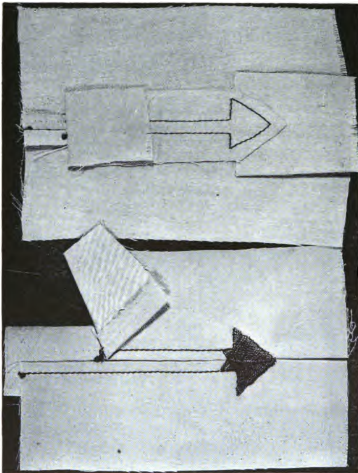
SLOT SEAM FINISHED WITH ARROW HEAD
